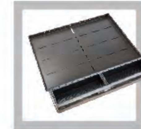
FLOWERY CUSTOMIZED Alu.Alloy | 1.0 mm Non-Stick Corrugated Bread Pan-8 Single Size: 366×115×140mm 362×111mm Ref. dough weight 1300g
