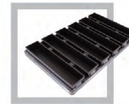
FLOWERY DZ222110151 Aluminium 6-strap Bread Pan-Black PTFE non-stick Size: 660×400×58.7mm Ref. dough weight 350g
