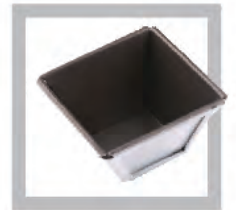
FLOWERY MY23511 Alu.Alloy | 1.0 mm Non-Stick Bread Pan (No Lid) Size: 95×95×60mm 55×55mm Ref. dough weight 80g
