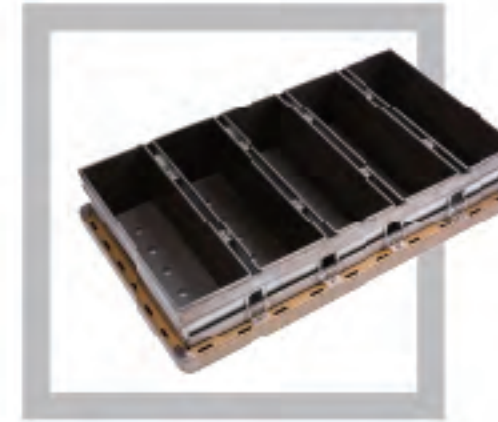
FLOWERY DZ217120171 Alusteel | 0.8/1.5 MM 5-Strap Non-Stick Corrugated Bread Pan Size: 375×121×140mm 365×119mm Ref. dough weight 1500g Patent No: ZL 2017 1 0018365.0
