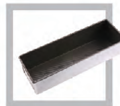
FLOWERY MY23411 Alu.Alloy | 1.0 mm Non-Stick Bread Pan Size: 360×115×90mm 356×111mm Ref. dough weight 900g
