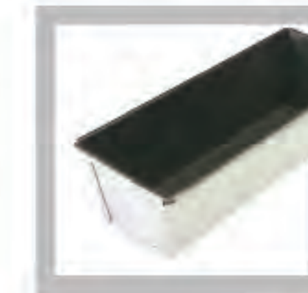
FLOWERY DZ2001 Alu.Alloy | 1.0 mm Non-Stick Bread Pan (No Lid) Size: 273×93×80mm 235×73mm Ref. dough weight 400-450g
