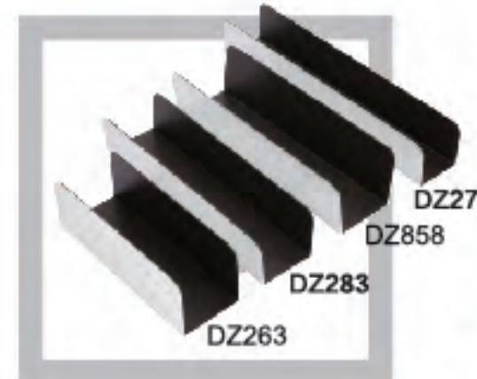
FLOWERY DZ273 Alu.Alloy | 1.5 mm Non-Stick Bread Pan-U Size: 245×40×40mm Ref. dough weight 100g
