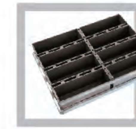
FLOWERY CUSTOMIZED Alu.Alloy | 1.0 mm Non-Stick Corrugated Bread Pan-8 (No Lid) Single Size: 366×115×90mm 361×111mm Ref. dough weight 900g
