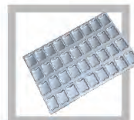
FLOWERY MY12322 Alusteel | 0.6/1.0 mm Mini Cake Tray Rabbit-36Cup (Silicone Glaze) Size: 600×400×25mm
