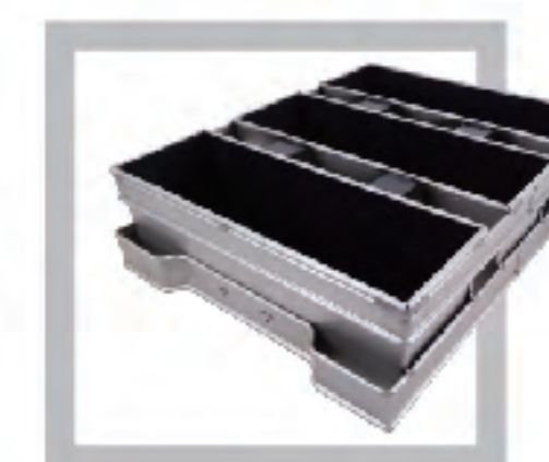
FLOWERY DZ22104005 Alusteel | 0.7/1.2 MM 3-strap 680g Loaf Pan Set-PTFE non-stick+heat painting Size: 400×297×115.7mm Ref. dough weight 680g
