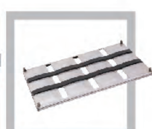
FLOWERY DZ221070161 Alusteel | 0.8/1.0/2.0/1.5 MM 4-Strap Loaf Pan-PTFE Non-Stick Inside+ Heat Painting Outer Long Side Size: 375×121×140mm 365×119mm Ref. dough weight 1500g
