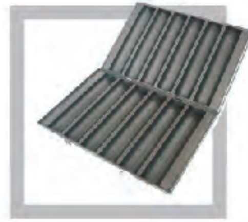
FLOWERY DZ2013 Alu.Alloy Non-Stick Round Bread Pan-6 Size: 600×400×83mm Ref. dough weight 2100g
